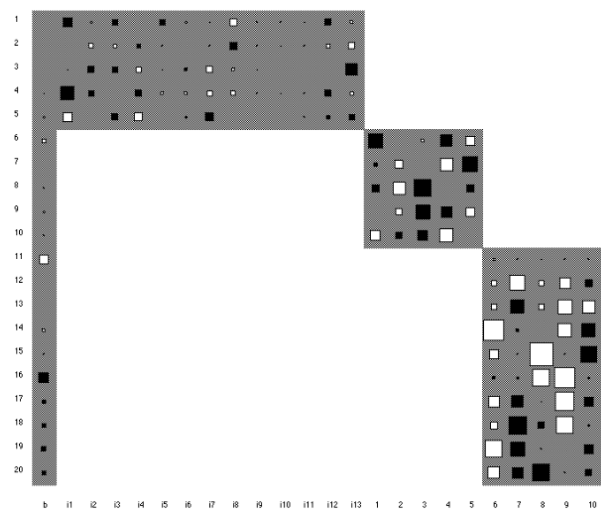
Fig. 9 Replication: Hinton Diagram (dark squares = inhibition, white squares = activation)
